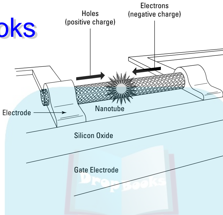
Figure 6-3: The carbon nanotube FET. The electrons come from the right (source), the holes come from the left (drain); they collide in the center, emitting light.
